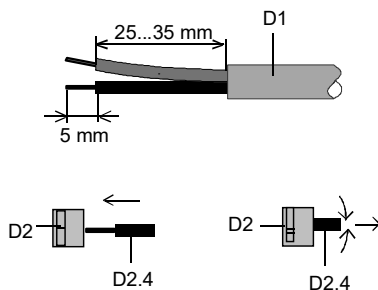
figure 6: Connecting / disconnecting bus cables
