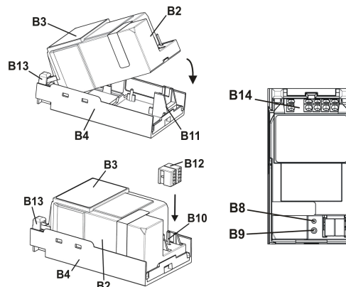
figure 3: Mounting of an RL module
