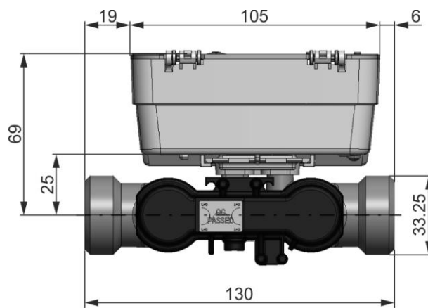
Fig. 8: Overview of dimensions mounting length 130 mm (threaded)
