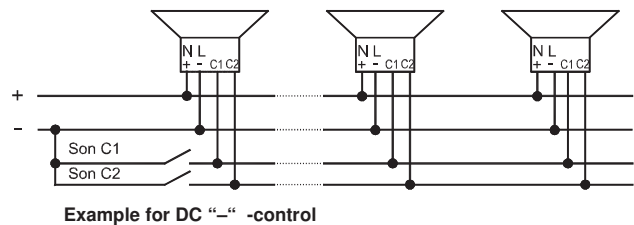
Exemple for DC “-“ -control
