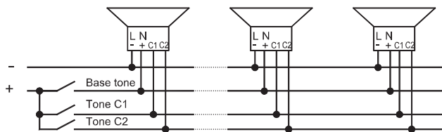
Connection example
