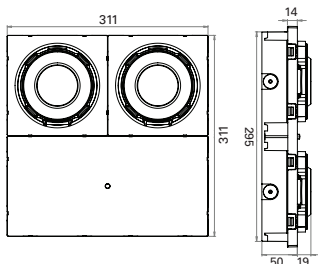
BeamTech 1000L - Dimensions (mm)
