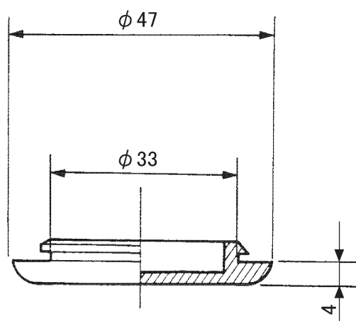
Drain cap
