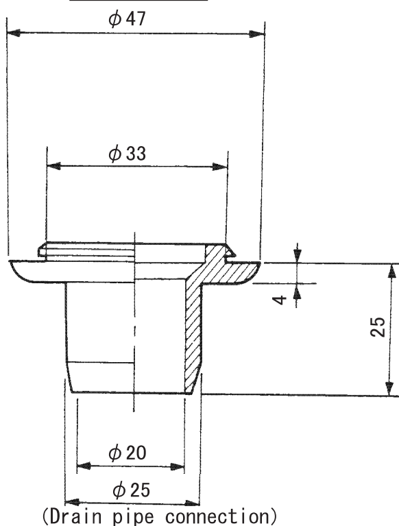
Drain socket
