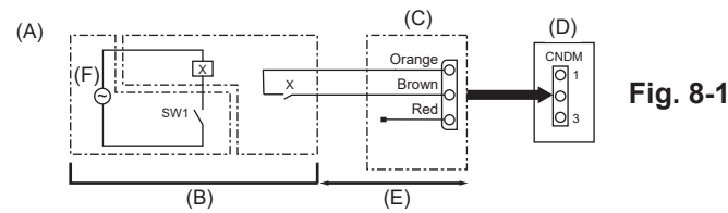
(A) Circuit diagram example (low noise mode) (D) Outdoor unit control board (B) On-site arrangement (E) Max. 10 m (C) External input adapter (PAC-SC36NA-E) (F) Power supply for relay X: Relay
