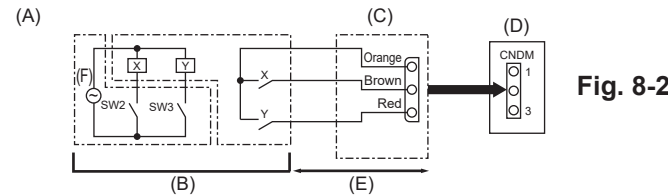
(A) Circuit diagram example (Demand function) (C) External input adapter (PAC-SC36NA-E) (B) On-site arrangement (D) Outdoor unit control board X, Y: Relay (E) Max. 10 m (F) Power supply for relay
