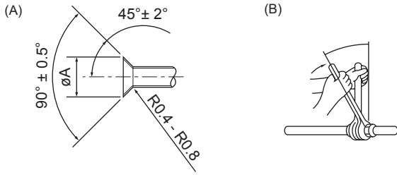
(A) Flare cutting dimensions (B) Flare nut tightening torque
