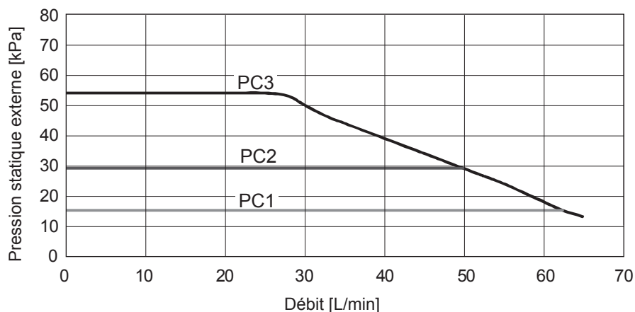
<Pression Constante>
