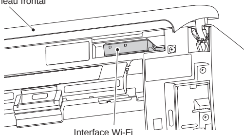
Interface Wi-Fi
