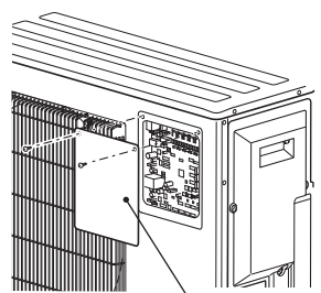
Maintenance panel
