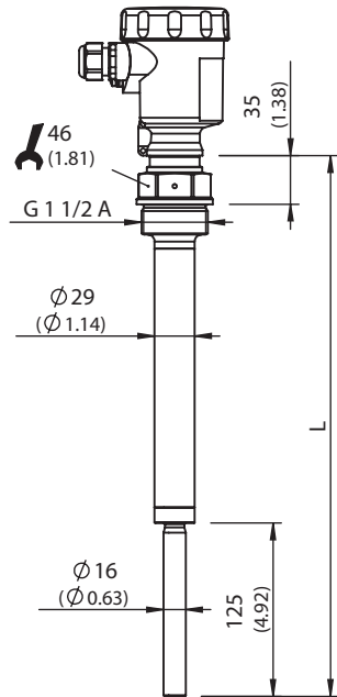
LBV331 threaded version G 1 ½ A
