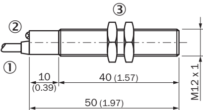
MM12 Namur, cable
