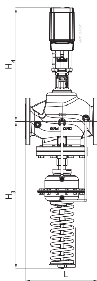
AMV(E) 55, 56/AFQMP 2 DN 65-125, PN 16/25/40
