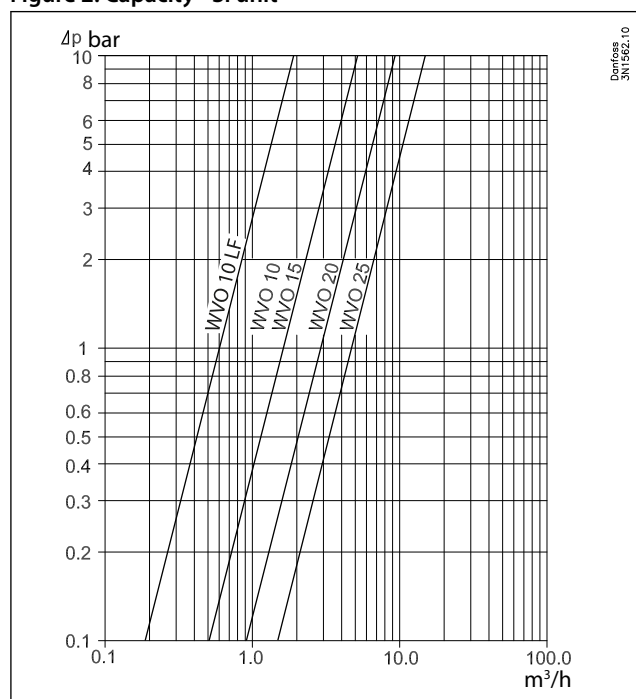
Figure 2: Capacity - SI unit
