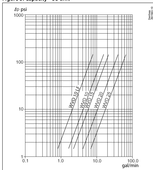
Figure 3: Capacity - US unit
