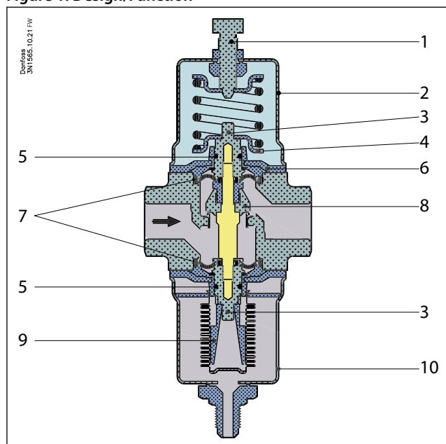
Figure 1: Design/Function
