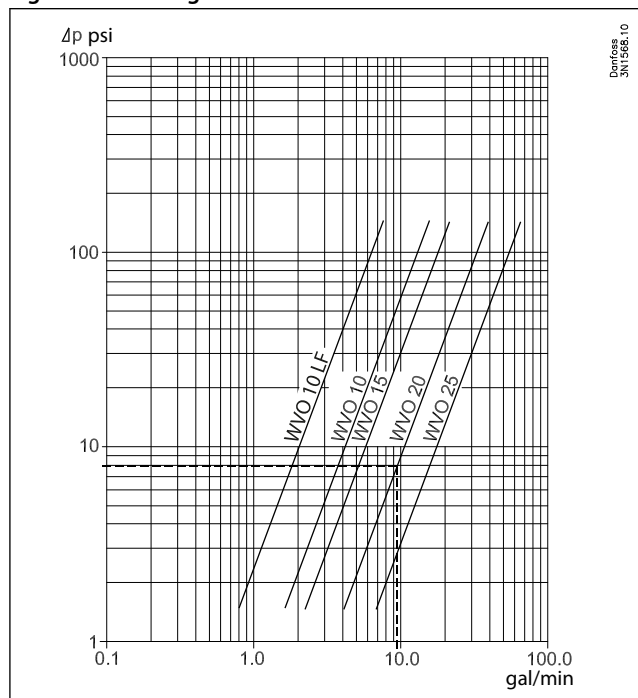
Figure 6: Selecting size - US units
