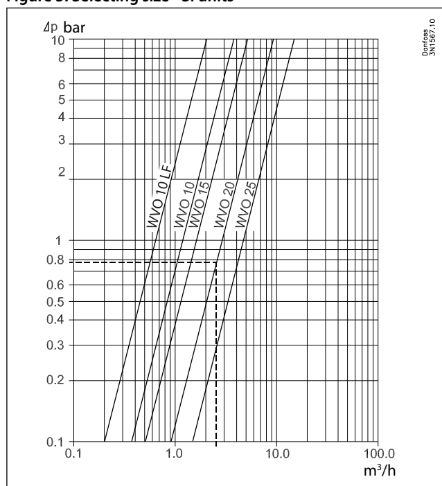
Figure 5: Selecting size - SI units
