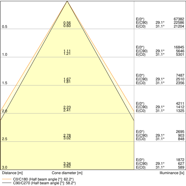
LB FLEX 1500 P 105W 840 N
