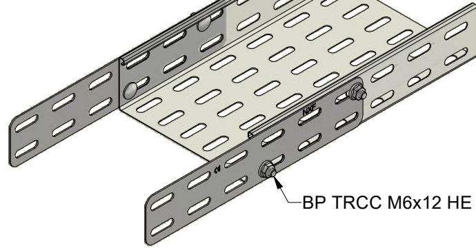
Dalle BD (BD Cable tray)
