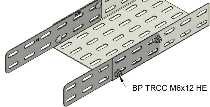
Dalle BD (BD Cable tray)
