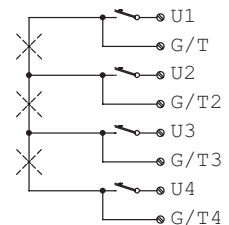
Button modules (Ref. 1145/12-13-14)
