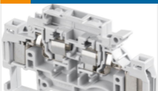
TE Part #1SNA199208R1100 D1.5/8.SFT.ADO
