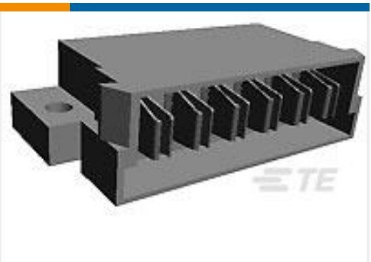
TE Part #6450129-7 MBXL R/A HDR STR 2P RAISED
