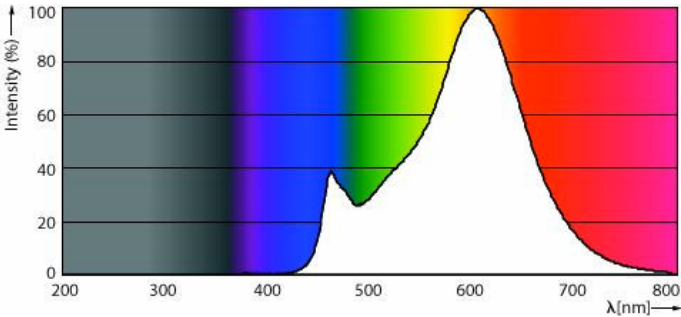
Spectral Power Distribution Colour - MZD LEDCLA 100W A60 E27 827 CL ND 1CT/10
