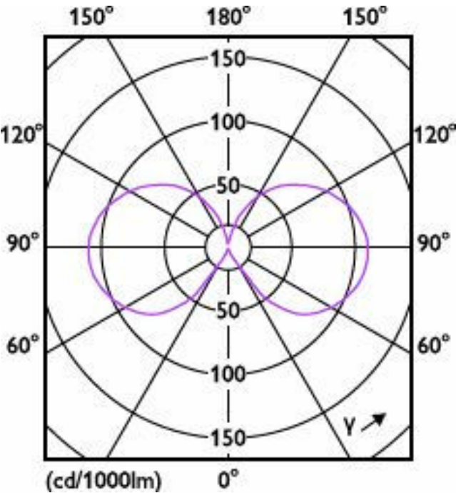
Light Distribution Diagram - MZD LEDCLA 100W A60 E27 827 CL ND 1CT/10
