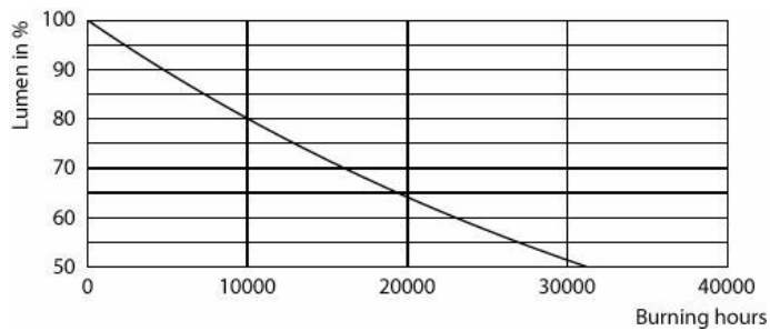
Lumen Maintenance Diagram - MZD LEDCLA 100W A60 E27 827 CL ND 1CT/10
