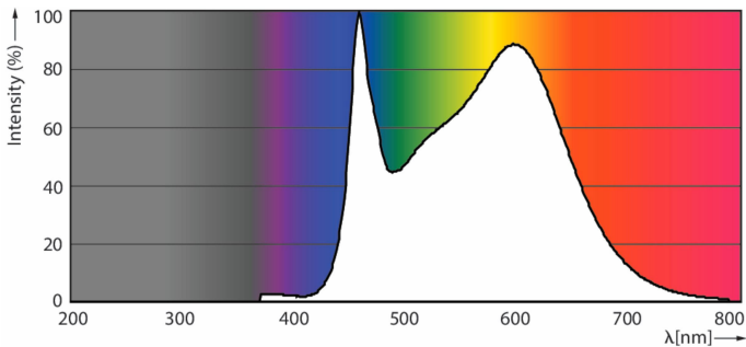
Spectral Power Distribution Colour - MZD LEDClassic 100W A60 E27 CWCLND1CT/10
