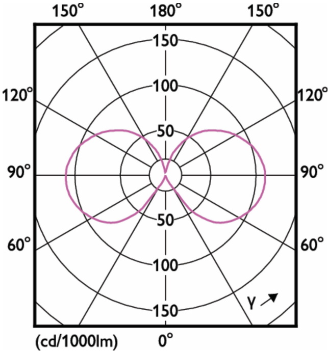
Light Distribution Diagram - MZD LEDClassic 100W A60 E27 CWCLND1CT/10
