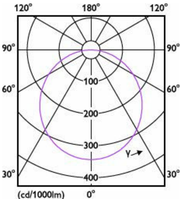
Light Distribution Diagram - MZD DN020B LED12/830 13W 220-240V D150
