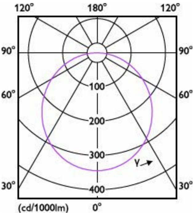
Light Distribution Diagram - MZD DN020B LED20/830 20W 220-240V D200
