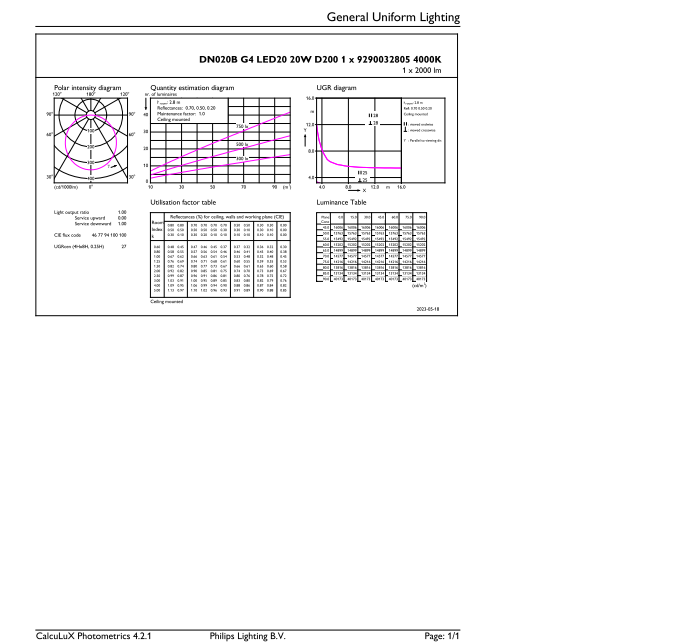
General uniform lighting - MZD DN020B LED20/840 20W 220-240V D200
