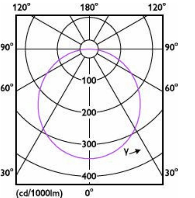
Light Distribution Diagram - MZD DN020B LED20/840 20W 220-240V D200
