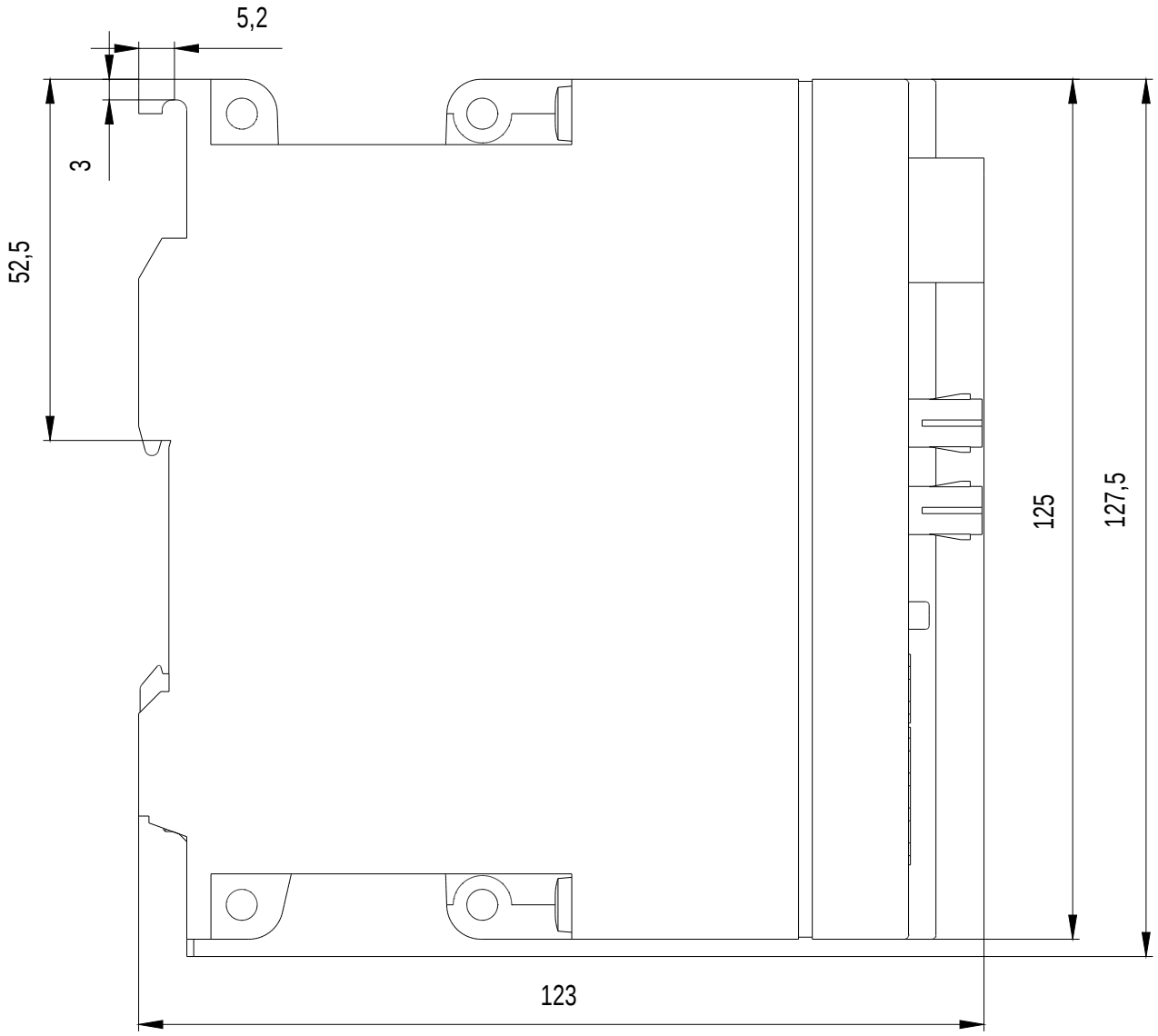
Links / Left
