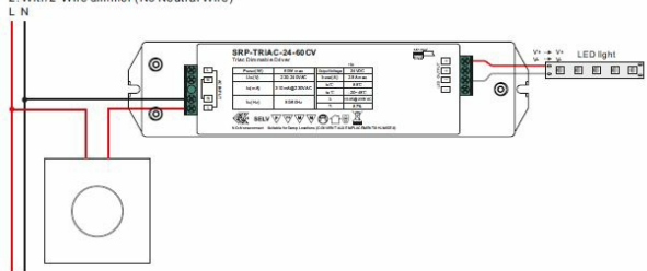
2. With 2-Wire dimmer (No Neutral Wire)
