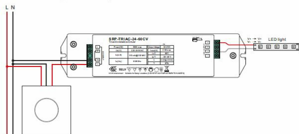
2. With 2-Wire dimmer (No Neutral Wire)
