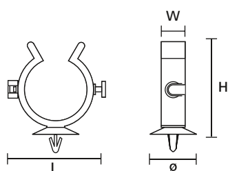
IPC Clip with arrowhead
