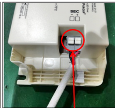
Figure3 Remove the wires
