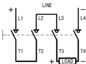
One-line control 4 poles in series
