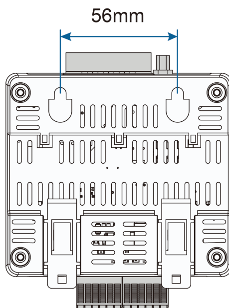
Figure 4-1 Trou de montage
