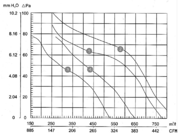
COURBE N°1 2E-200-9 220V/50Hz 0~90Pa (20Pa-710m 3 /h)
