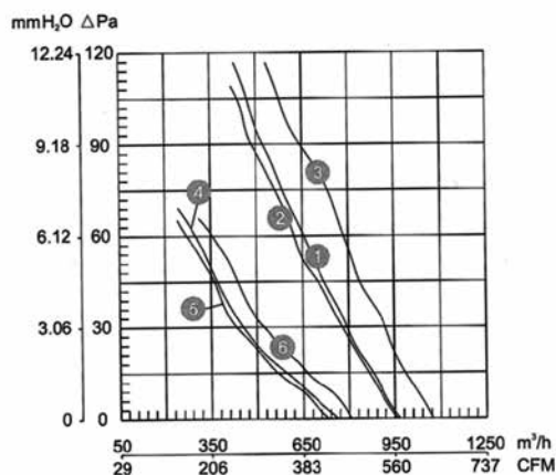
COURBE N°1 2D-250 380V/50Hz 0~90Pa (20Pa-850m 3 /h)
