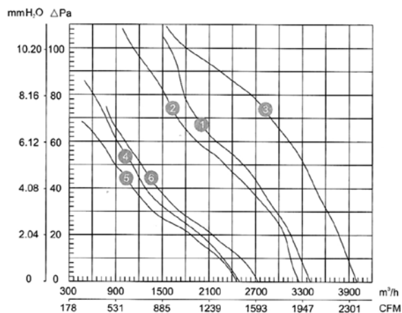
COURBE N°4 6D-350 380V/50Hz 0-60Pa (20Pa-1980m 3 /h)
