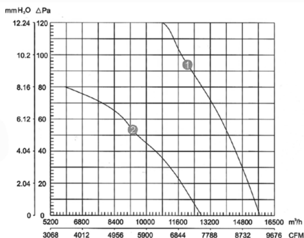
■ COURBE N°2 6E-710 Y380V/50Hz 0~120Pa (20Pa-11680m 3 /h)
