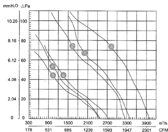
COURBE N°1 4D-400 380V/50Hz 0~90Pa (20Pa-3150m 3 /h)
