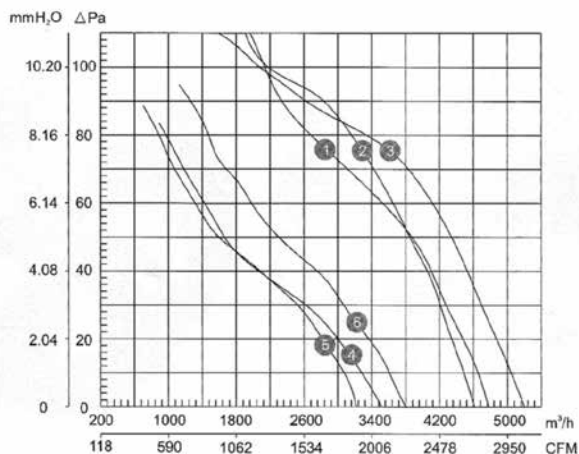
COURBE N°1 4D-450 380V/50Hz 0~90Pa (20Pa-4450m 3 /h)
