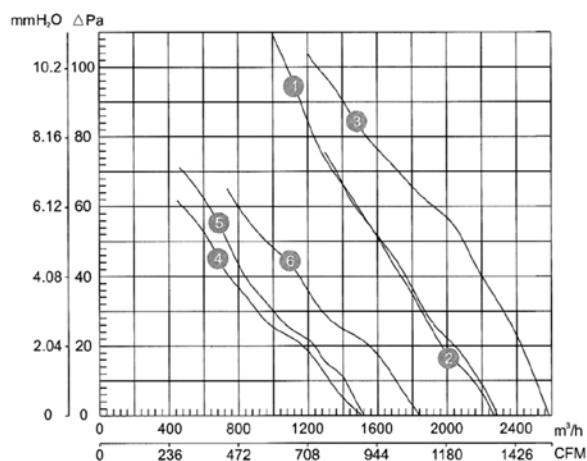
■ COURBE N°5 6E-350 220V/50Hz 0-60Pa (20Pa-1170m 3 /h)
