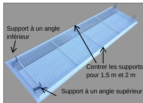
Fig. 5b: grille plus large
