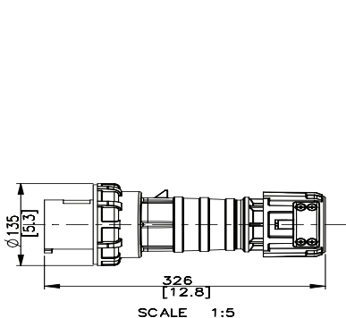
Plug
