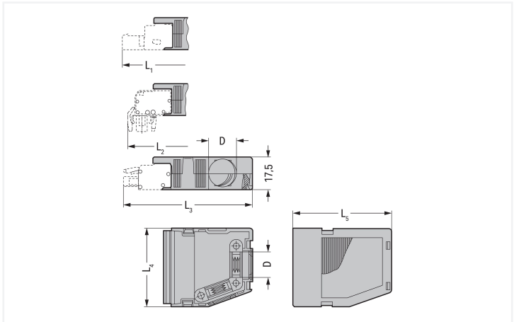
Dimensions en mm 2- to 3-pole; only suitable for cable ties; 1 cable outlet (rear side); max. 3.6 mm cable tie width4- to 6-pole; suitable for cable clamp; 1 x cable outlet (rear side)7- to 8-pole; suitable for cable clamp; 1 x cable outlet (rear side) and 1 x cable outlet (side); 1 cover (included)9- to 16-pole; suitable for cable clamp; 1 x cable outlet (rear side) and 2 x cable outlets (side); 2 covers (included)Cable ties and binding tools are not offered by WAGO.
