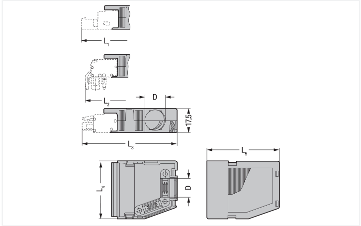
Dimensions en mm D = Ø câble max. 14 mm L1= 71,5 mm L2= 68,0 mm L3= 70,5 mm L4= 85,0 mm L5= 54,0 mm
