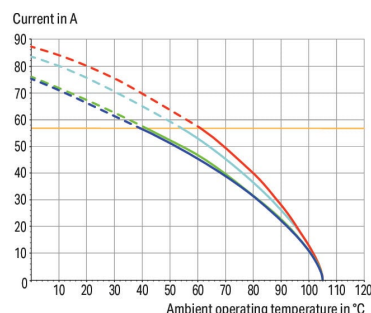
Current-carrying capacity curve PCB terminal block (2626-31xx/0020-0000) Pin spacing: 7.5 mm / Conductor cross-section: 10 mm 2 "f-st" Based on: EN 60512-5-2 / Reduction factor: 1
