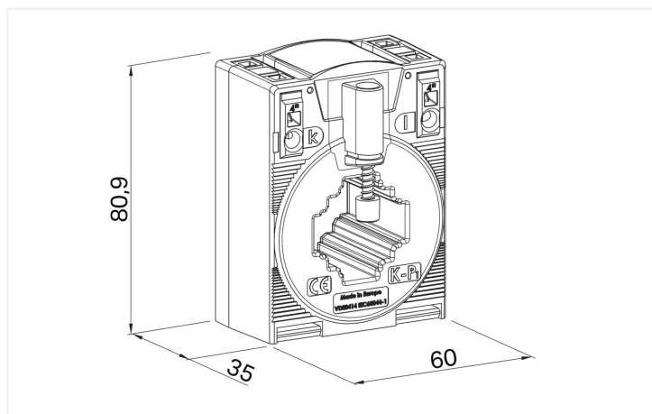
Short description: WAGO's plug-in current transformers for billing measurement (855 Series) are inductive, single-conductor current transformers. Due to the measurement principle used, these current transformers are exclusively designed for AC network applications. These plug-in current transformers comply with the conformity assessment procedure (module D) and can be used for billing purposes in Germany (MessEG).
