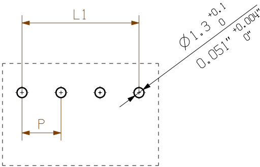
HOLE PATTERN
