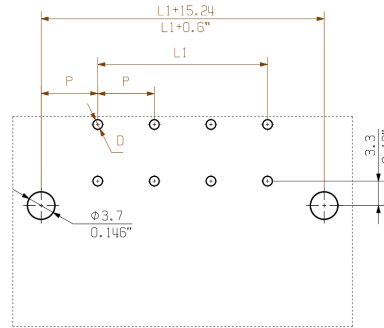
hole pattern
