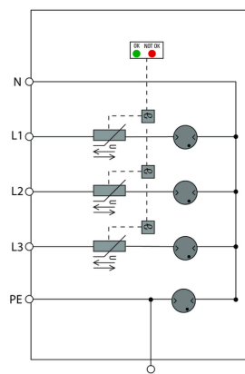
Circuit diagram
