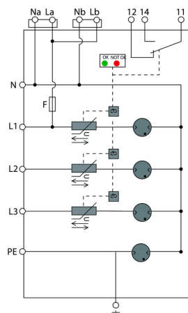
Circuit diagram
