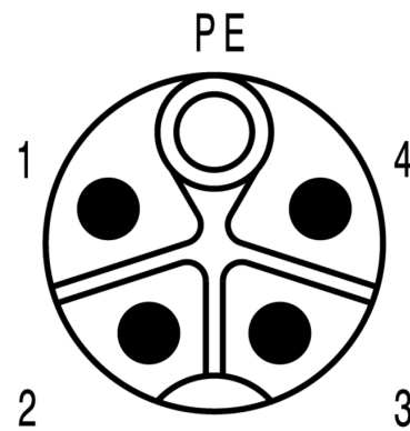
Plug
