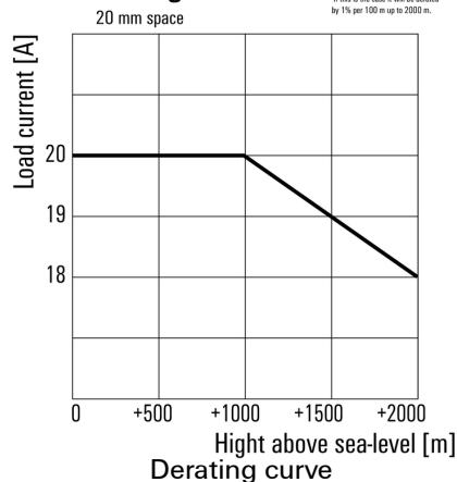
Derating curve
