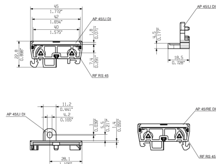
DIRECT MOUNTING
